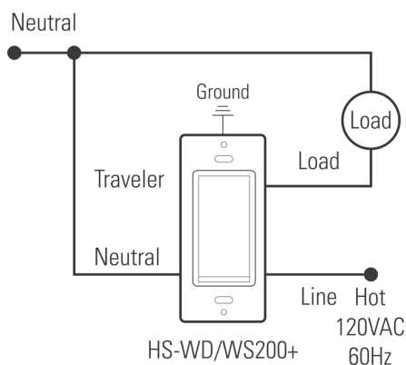
Single-pole circuit
