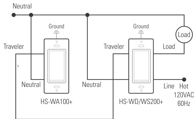
3-way circuit
