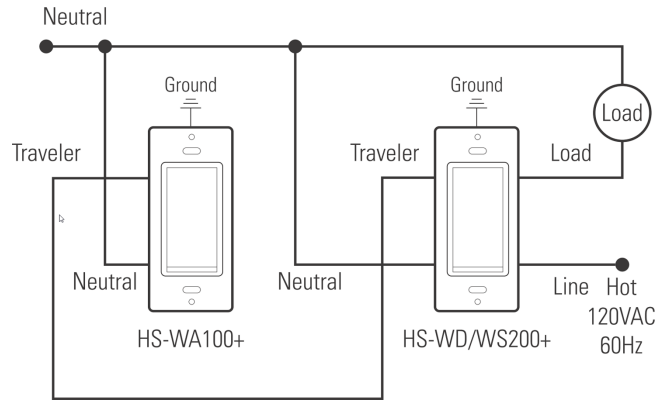
3-way circuit
